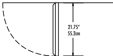
DOOR CLEARANCE DETAIL
